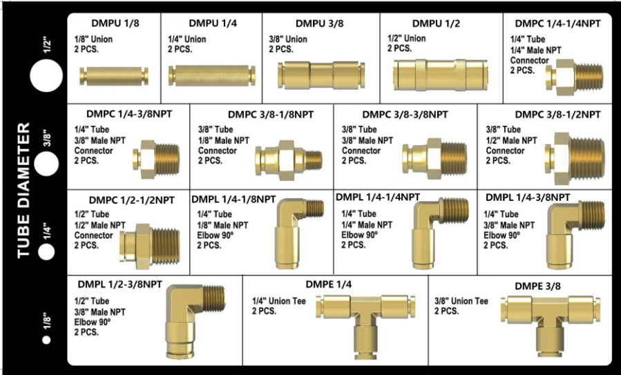
DOT Air Brake Brass Push to Connect Kit (1/4", 3/8", & 1/2") 32 pcs
